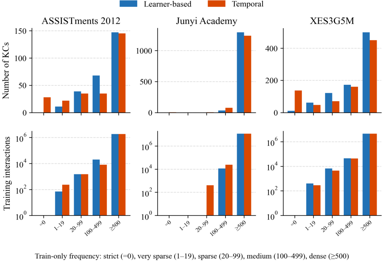
Fig. 2. Distribution of KCs across train-only frequency strata under learner-based and temporal splits. Bottom: verified training-interaction counts (sum of train-only ftrain on fold 0); volume is not inferred from KC counts. Bottom y-axis is logarithmic.
